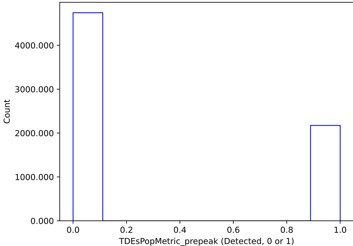
too_elab_r8_d2_giz_v3.4_10yrs : TDEsPopMetric_prepeak
