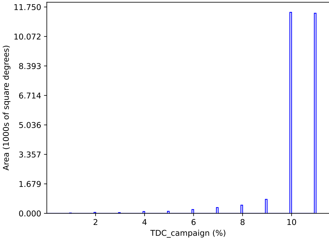
too_elab_r8_d2_giz_v3.4_10yrs : TDC_campaign
