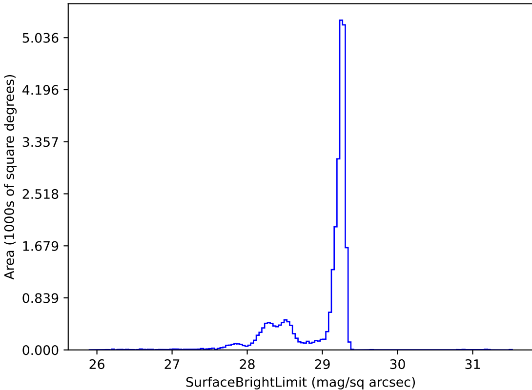
too_elab_r8_d2_giz_v3.4_10yrs z: SurfaceBrightLimit
