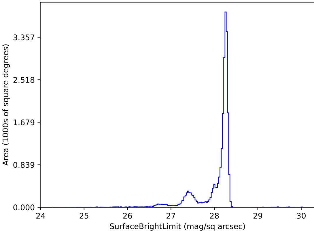
too_elab_r8_d2_giz_v3.4_10yrs y: SurfaceBrightLimit
