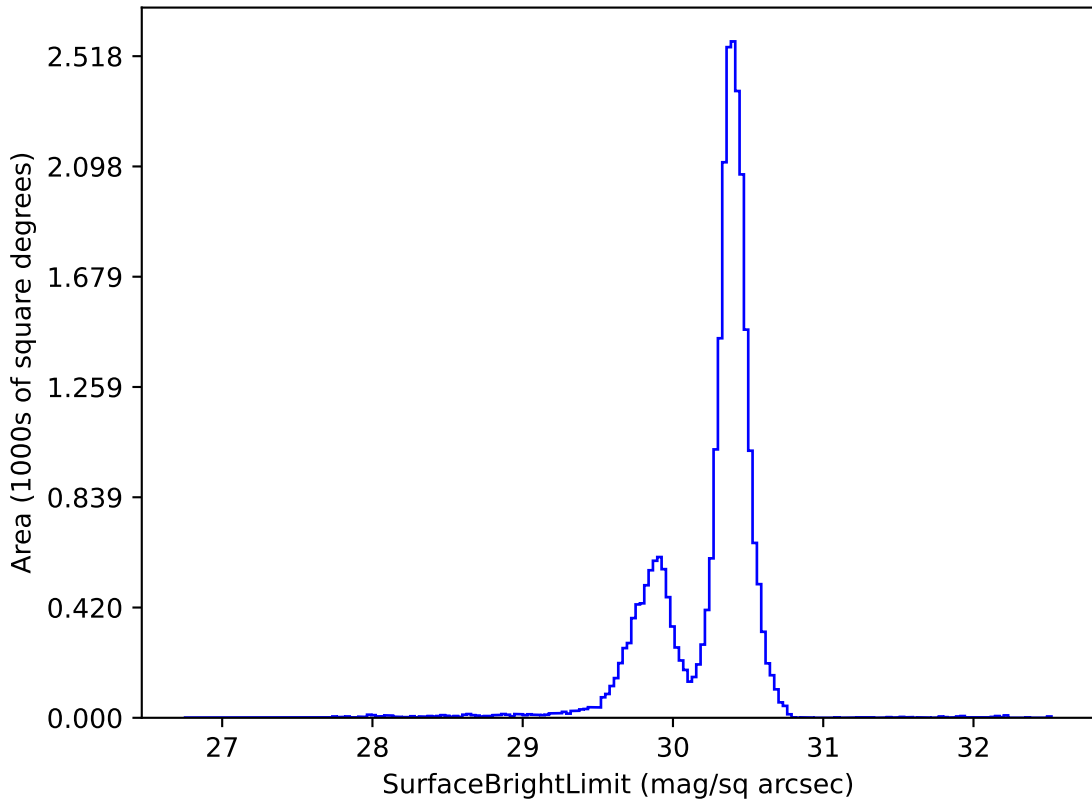
too_elab_r8_d2_giz_v3.4_10yrs g: SurfaceBrightLimit
