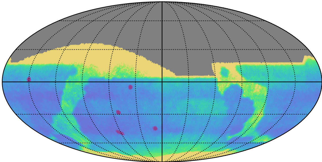
too_elab_r8_d2_giz_v3.4_10yrs : Proper Motion Uncert @ 24.0
