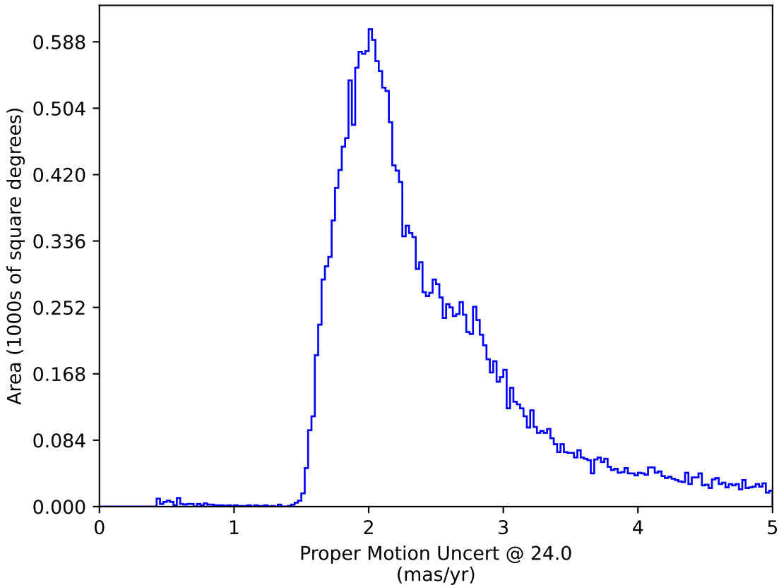
too_elab_r8_d2_giz_v3.4_10yrs : Proper Motion Uncert @ 24.0
