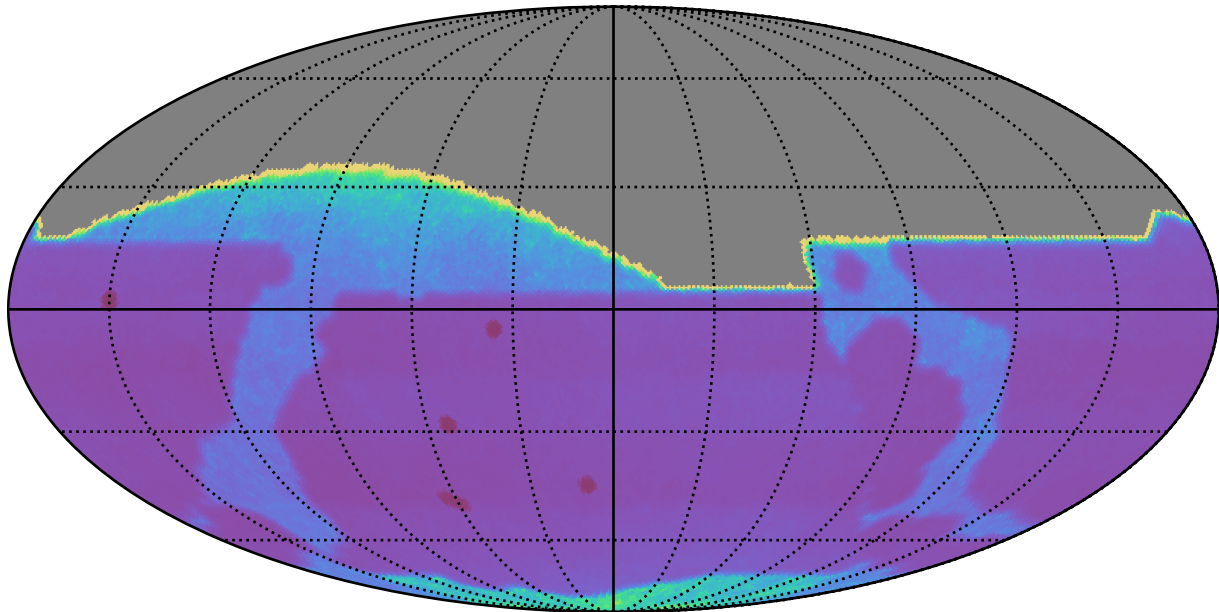
too_elab_r8_d2_giz_v3.4_10yrs : Proper Motion Uncert @ 20.5
