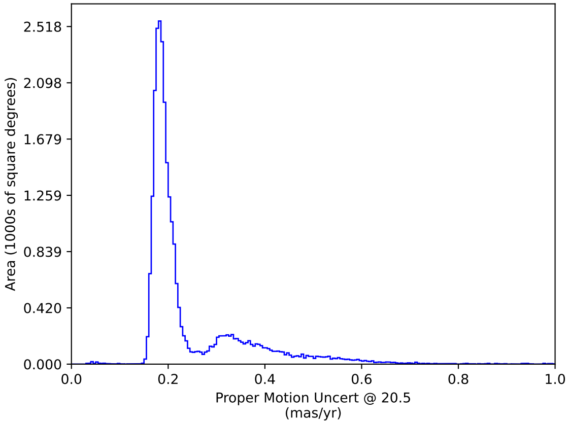
too_elab_r8_d2_giz_v3.4_10yrs : Proper Motion Uncert @ 20.5
