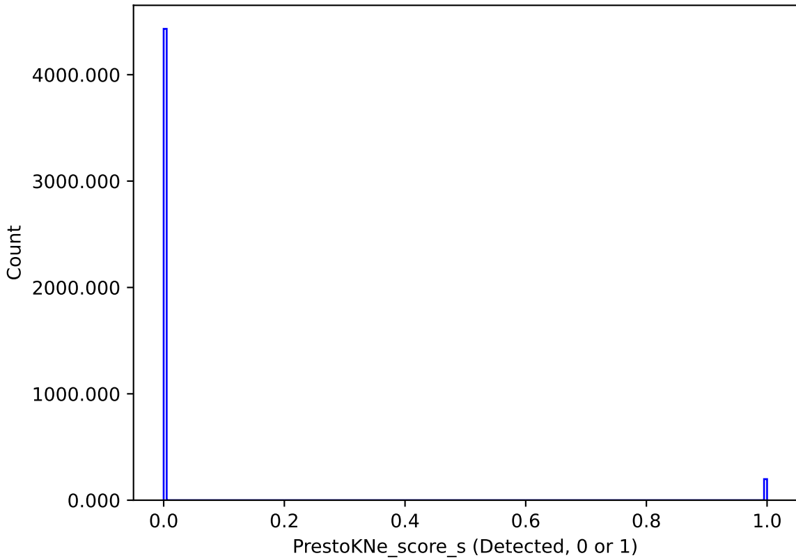
too_elab_r8_d2_giz_v3.4_10yrs : PrestoKNe_score_s
