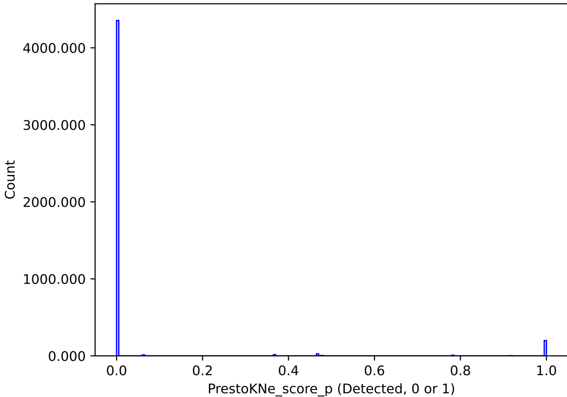
too_elab_r8_d2_giz_v3.4_10yrs : PrestoKNe_score_p
