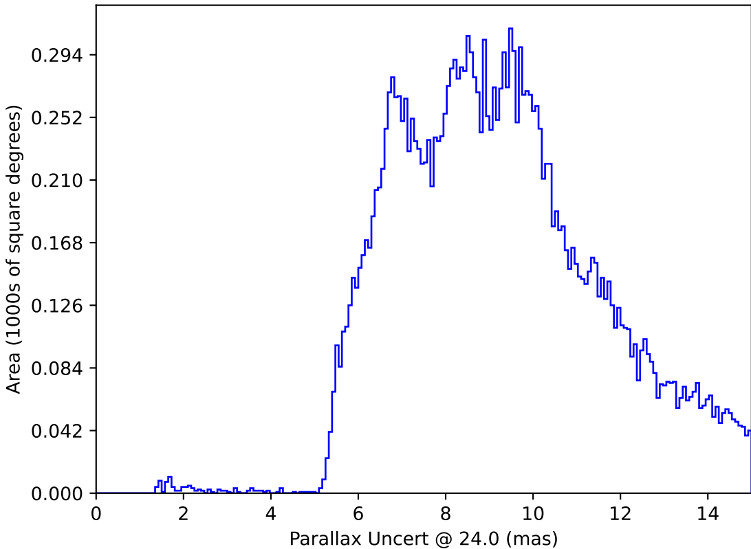
too_elab_r8_d2_giz_v3.4_10yrs : Parallax Uncert @ 24.0
