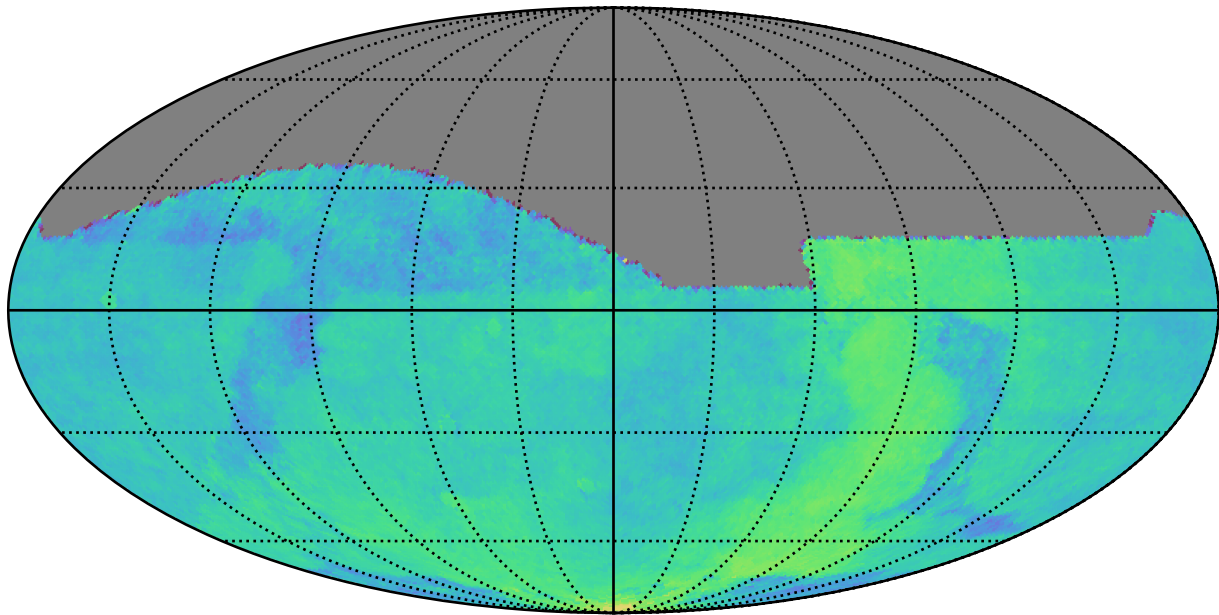
too_elab_r8_d2_giz_v3.4_10yrs : Parallax Coverage @ 24.0
