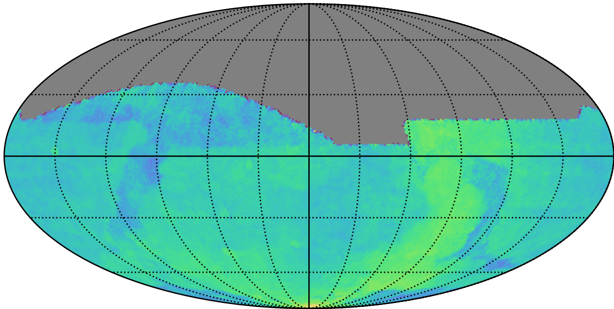
too_elab_r8_d2_giz_v3.4_10yrs : Parallax Coverage @ 22.4
