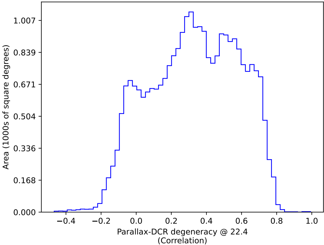
too_elab_r8_d2_giz_v3.4_10yrs : Parallax-DCR degeneracy @ 22.4
