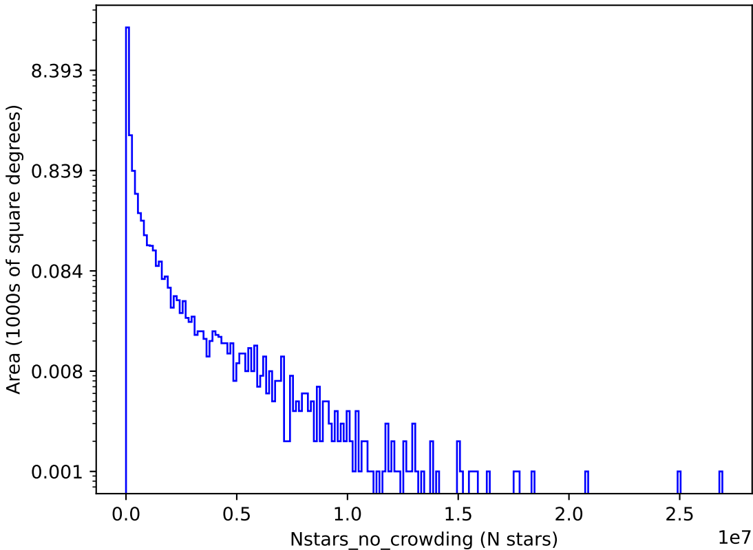
too_elab_r8_d2_giz_v3.4_10yrs z: Nstars_no_crowding
