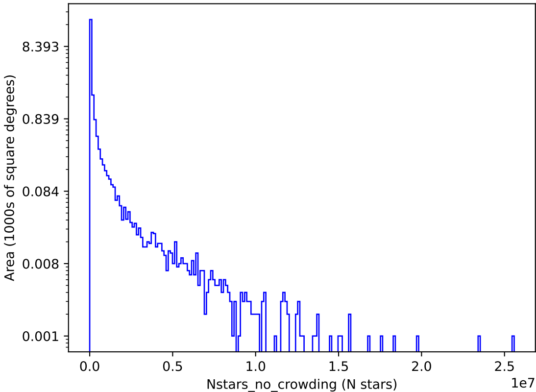
too_elab_r8_d2_giz_v3.4_10yrs y: Nstars_no_crowding
