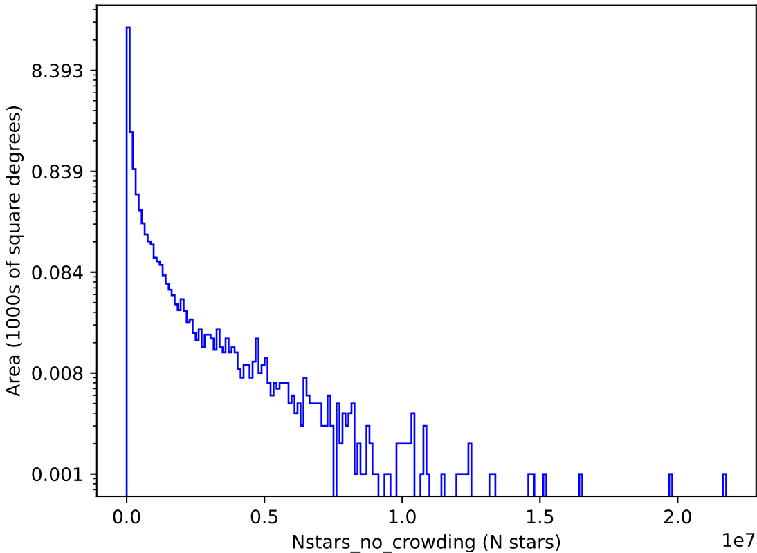
too_elab_r8_d2_giz_v3.4_10yrs r: Nstars_no_crowding
