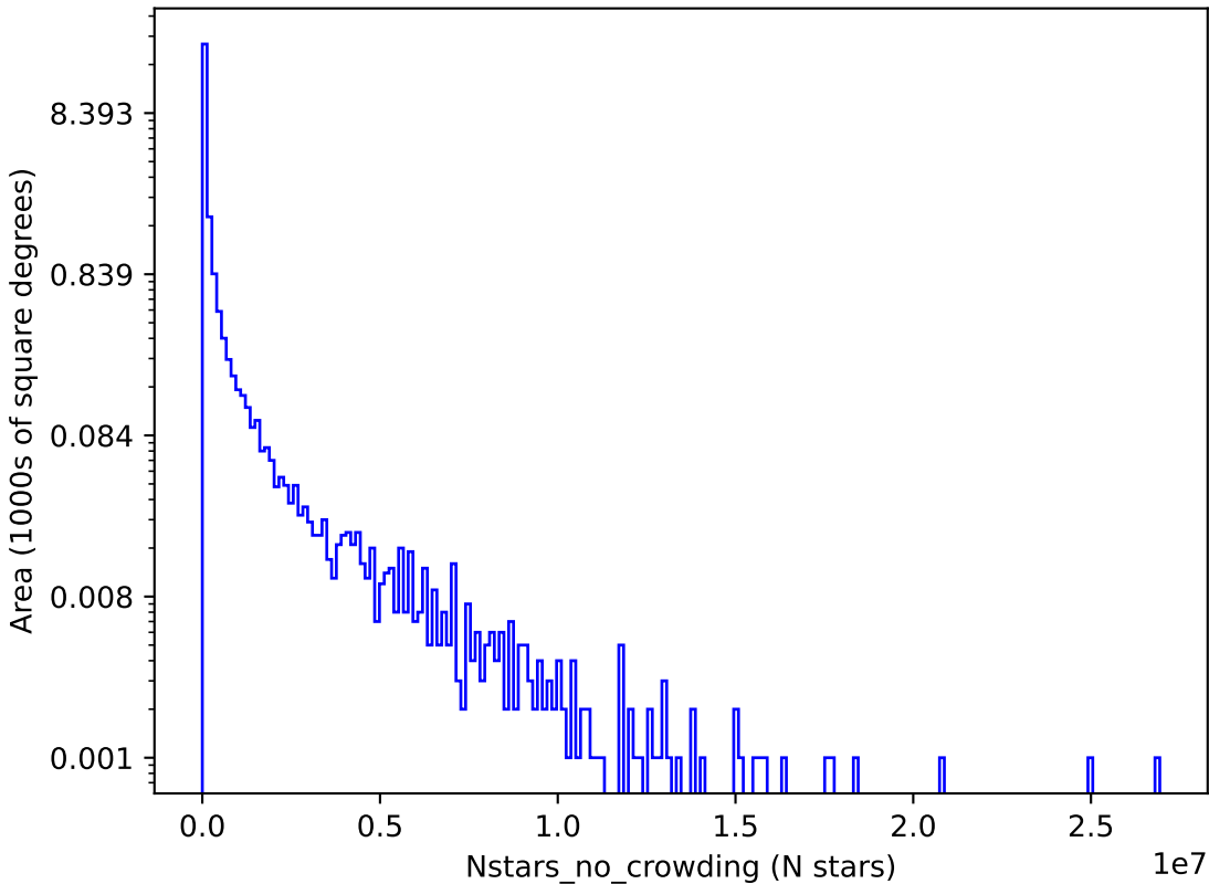
too_elab_r8_d2_giz_v3.4_10yrs i: Nstars_no_crowding
