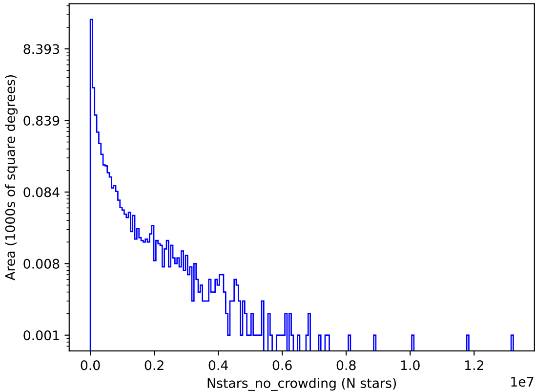
too_elab_r8_d2_giz_v3.4_10yrs g: Nstars_no_crowding
