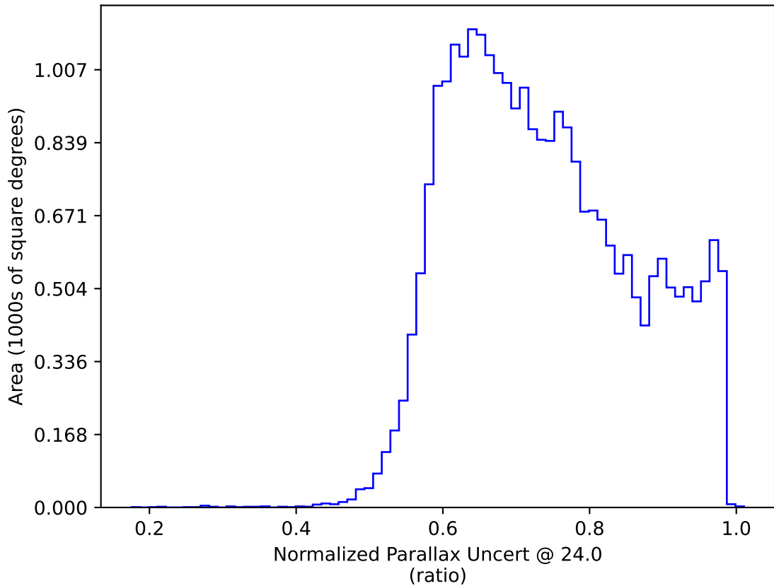
too_elab_r8_d2_giz_v3.4_10yrs : Normalized Parallax Uncert @ 24.0
