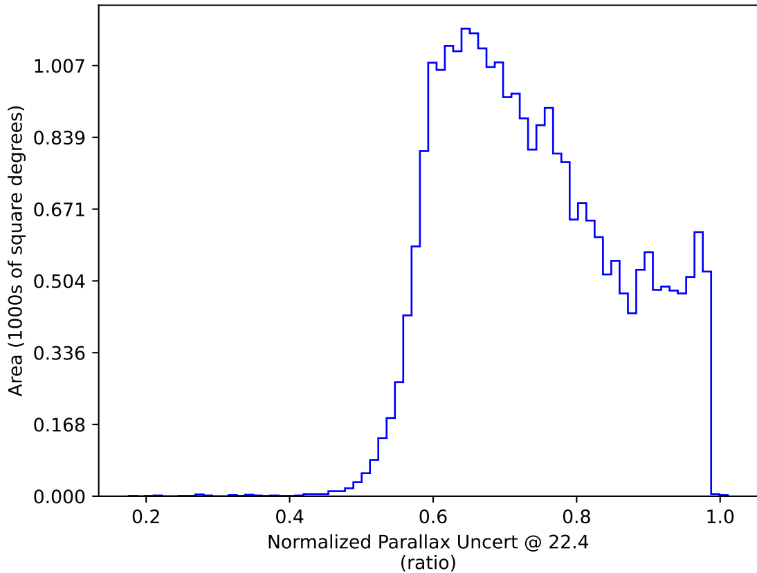
too_elab_r8_d2_giz_v3.4_10yrs : Normalized Parallax Uncert @ 22.4
