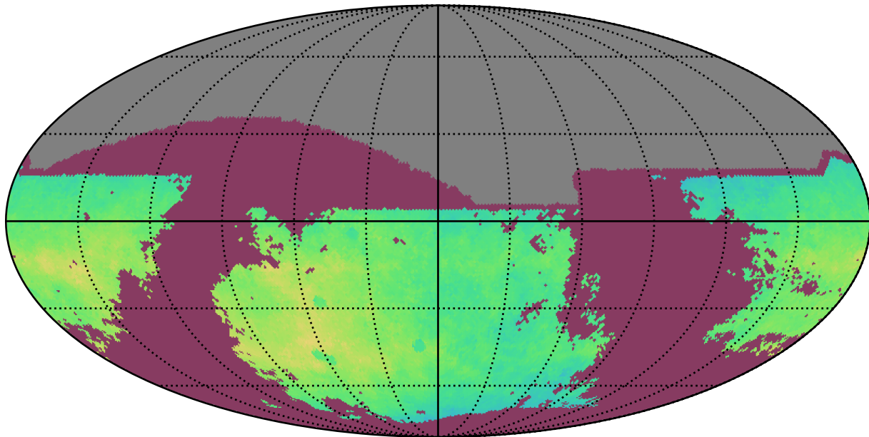
too_elab_r8_d2_giz_v3.4_10yrs i: NgalScale
