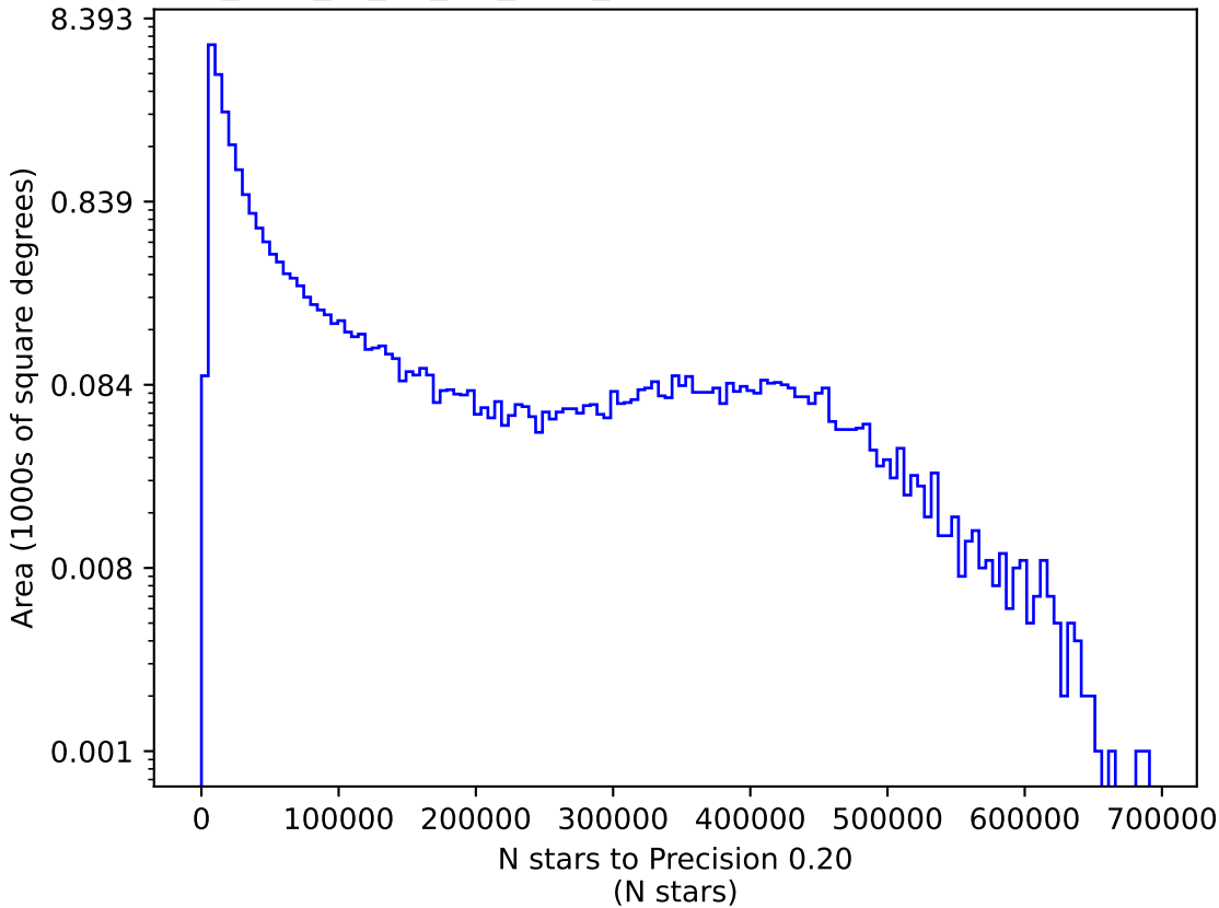
too_elab_r8_d2_giz_v3.4_10yrs z: N stars to Precision 0.20
