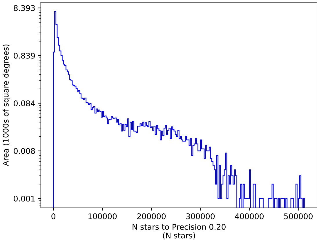
too_elab_r8_d2_giz_v3.4_10yrs u: N stars to Precision 0.20
