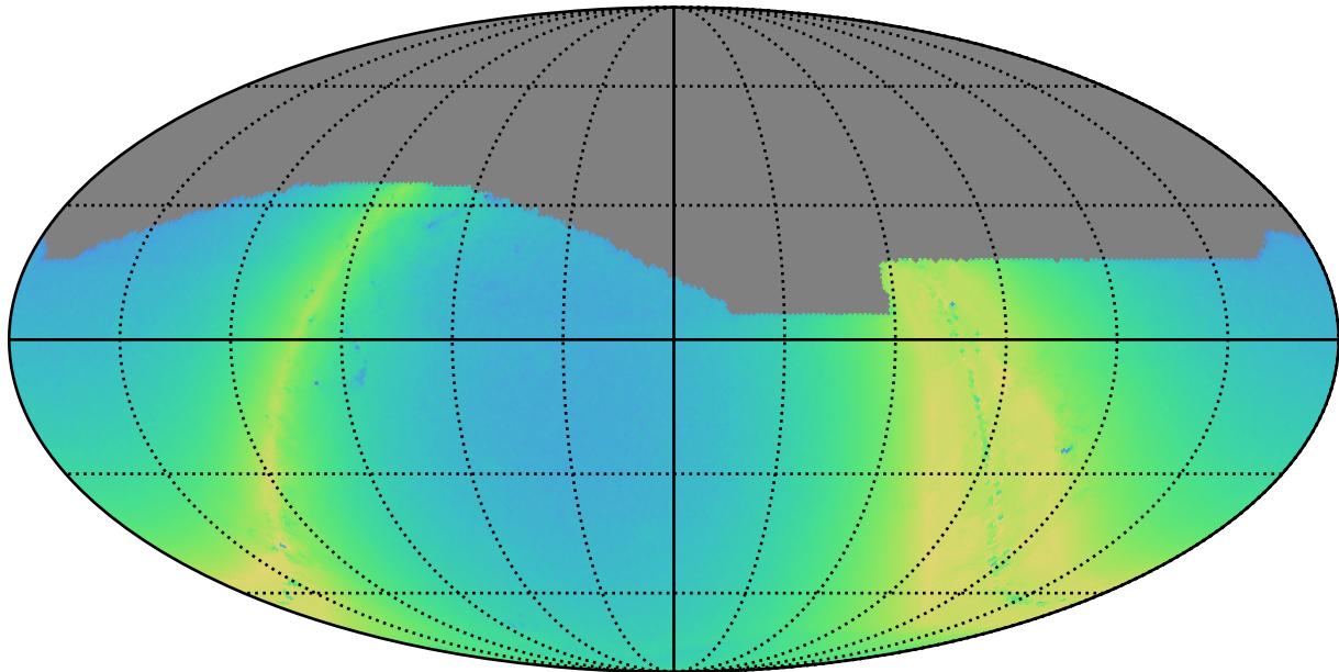
too_elab_r8_d2_giz_v3.4_10yrs r: N stars to Precision 0.20
