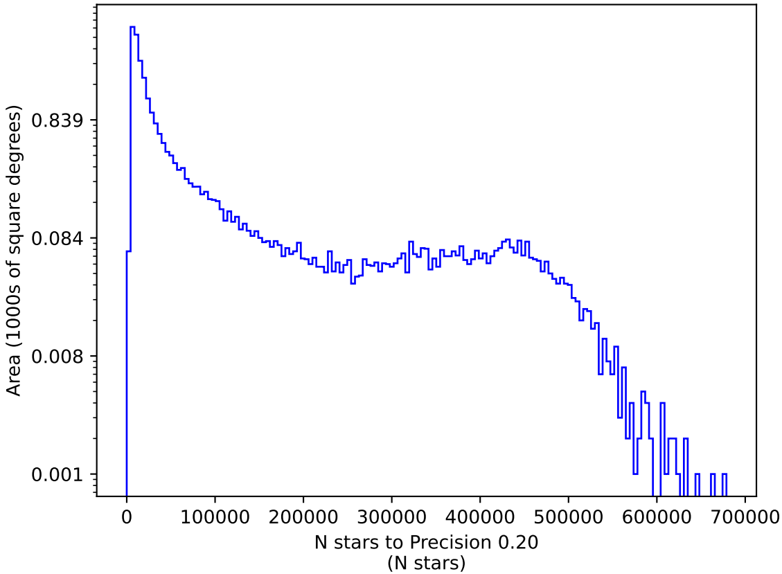
too_elab_r8_d2_giz_v3.4_10yrs r: N stars to Precision 0.20
