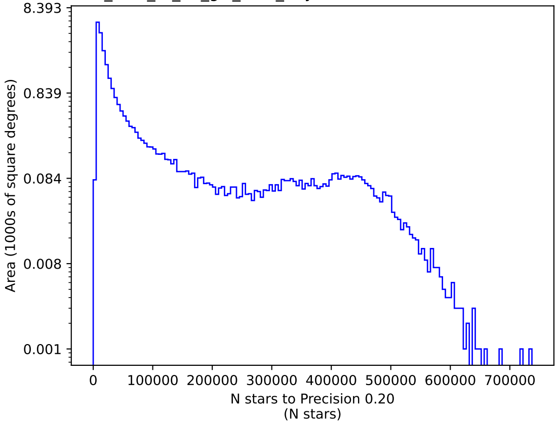
too_elab_r8_d2_giz_v3.4_10yrs i: N stars to Precision 0.20
