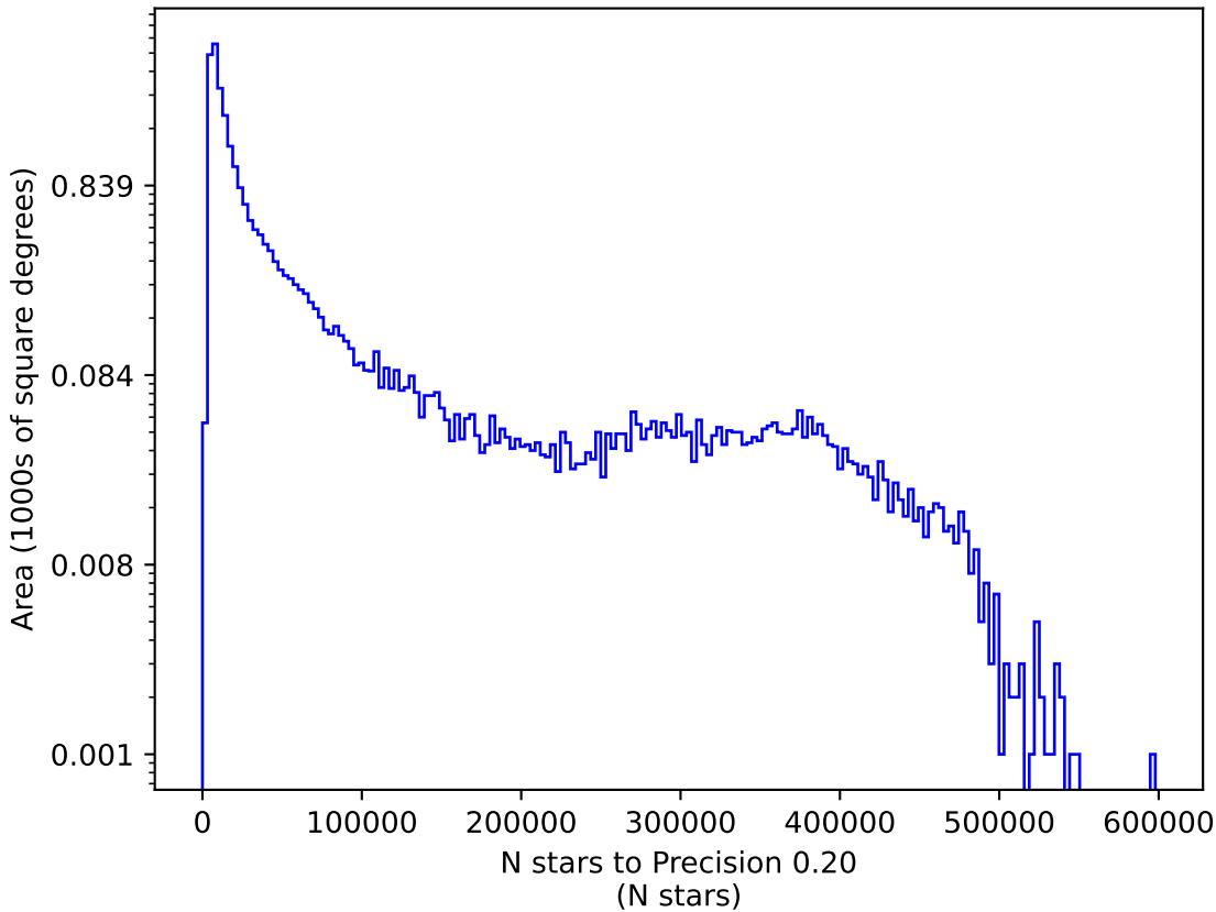
too_elab_r8_d2_giz_v3.4_10yrs g: N stars to Precision 0.20
