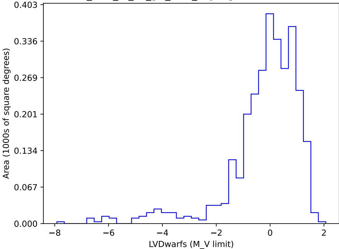
too_elab_r8_d2_giz_v3.4_10yrs gi SCP: LVDwarfs
