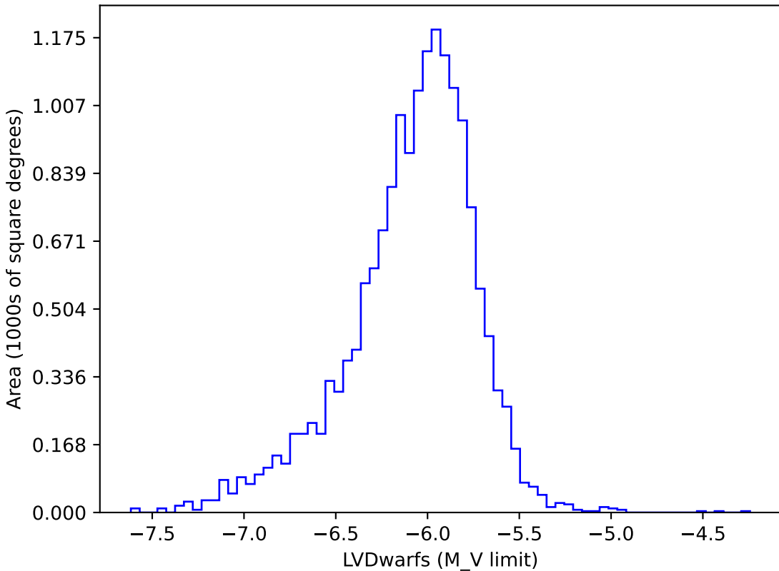
too_elab_r8_d2_giz_v3.4_10yrs gi: LVDwarfs
