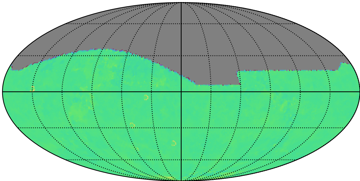
too_elab_r8_d2_giz_v3.4_10yrs z: Kuiper rotTelPos
