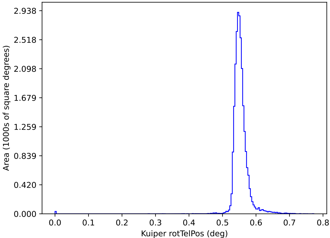
too_elab_r8_d2_giz_v3.4_10yrs y: Kuiper rotTelPos
