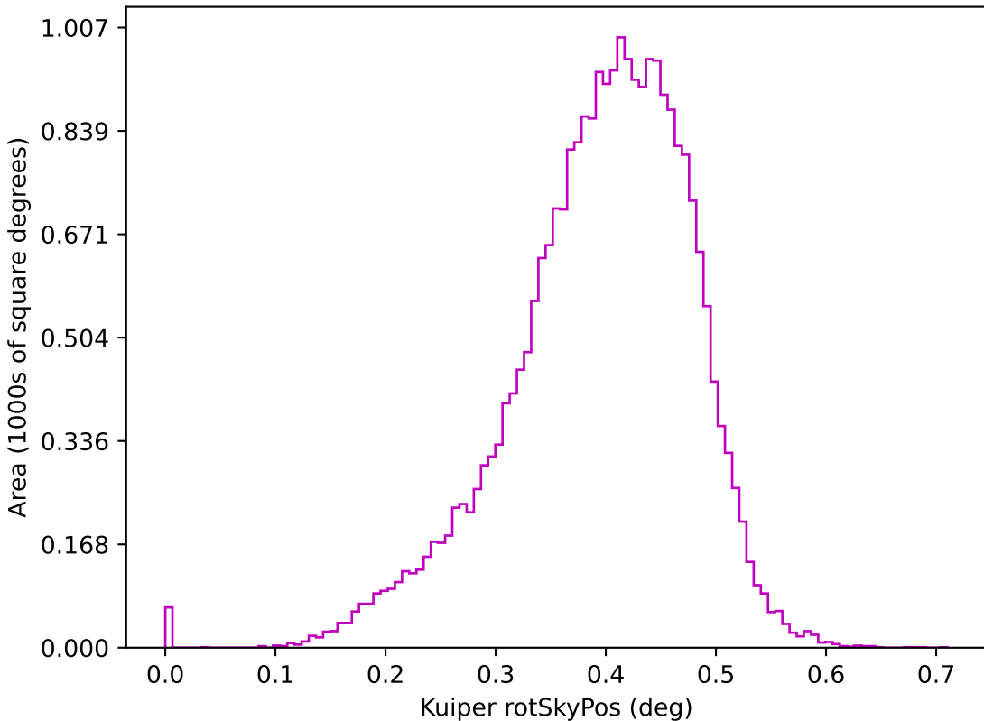
too_elab_r8_d2_giz_v3.4_10yrs z: Kuiper rotSkyPos
