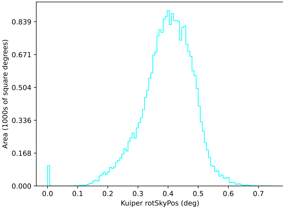
too_elab_r8_d2_giz_v3.4_10yrs u: Kuiper rotSkyPos
