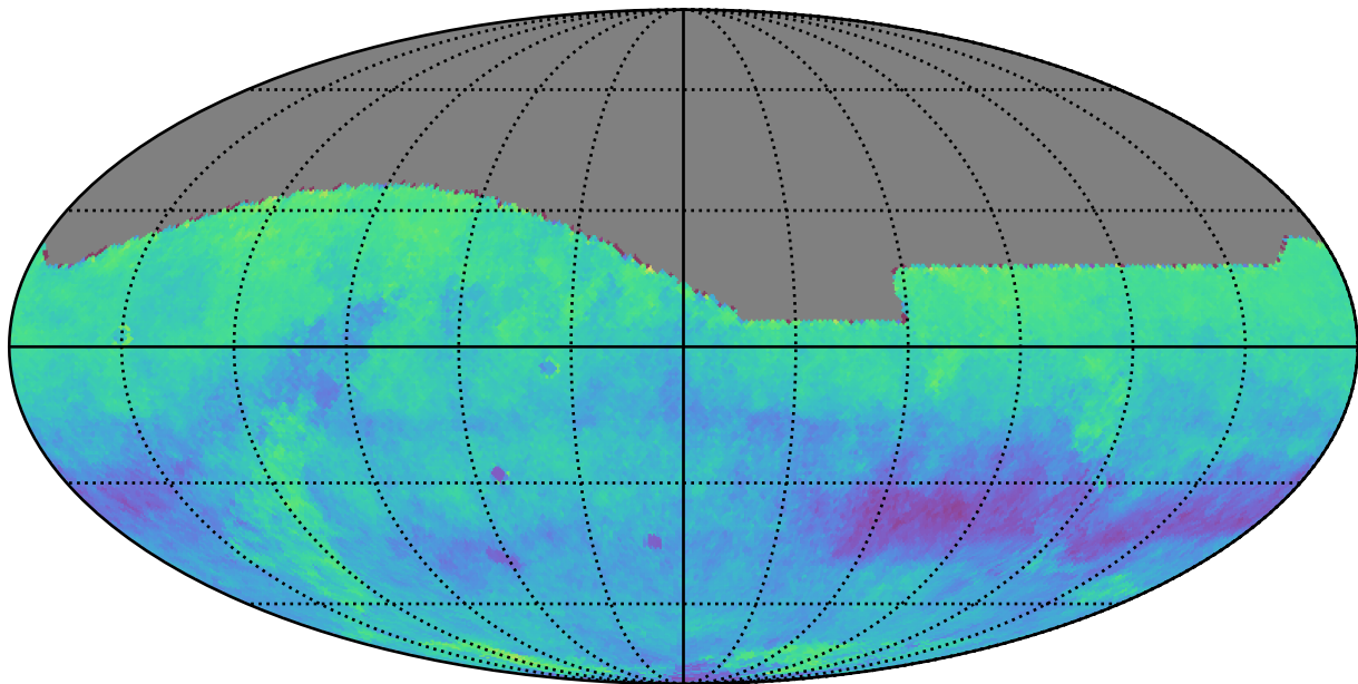
too_elab_r8_d2_giz_v3.4_10yrs r: Kuiper rotSkyPos
