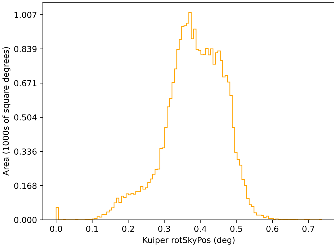
too_elab_r8_d2_giz_v3.4_10yrs r: Kuiper rotSkyPos
