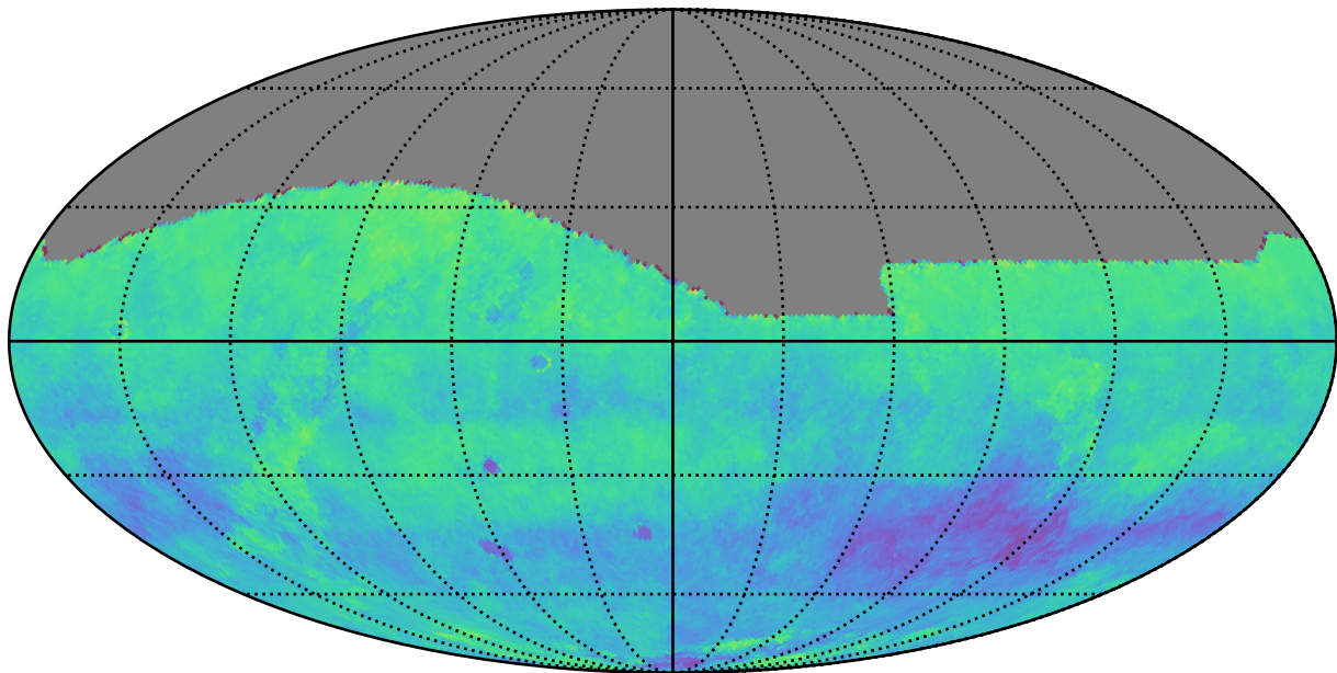
too_elab_r8_d2_giz_v3.4_10yrs i: Kuiper rotSkyPos
