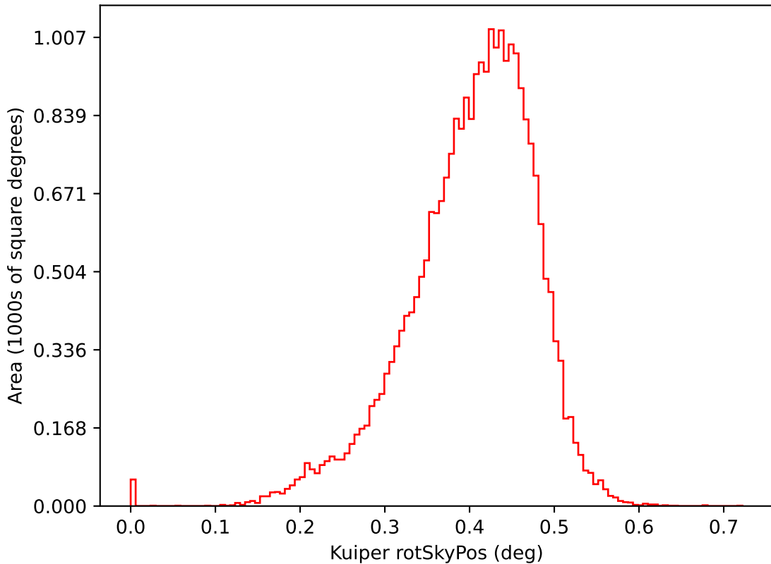
too_elab_r8_d2_giz_v3.4_10yrs i: Kuiper rotSkyPos
