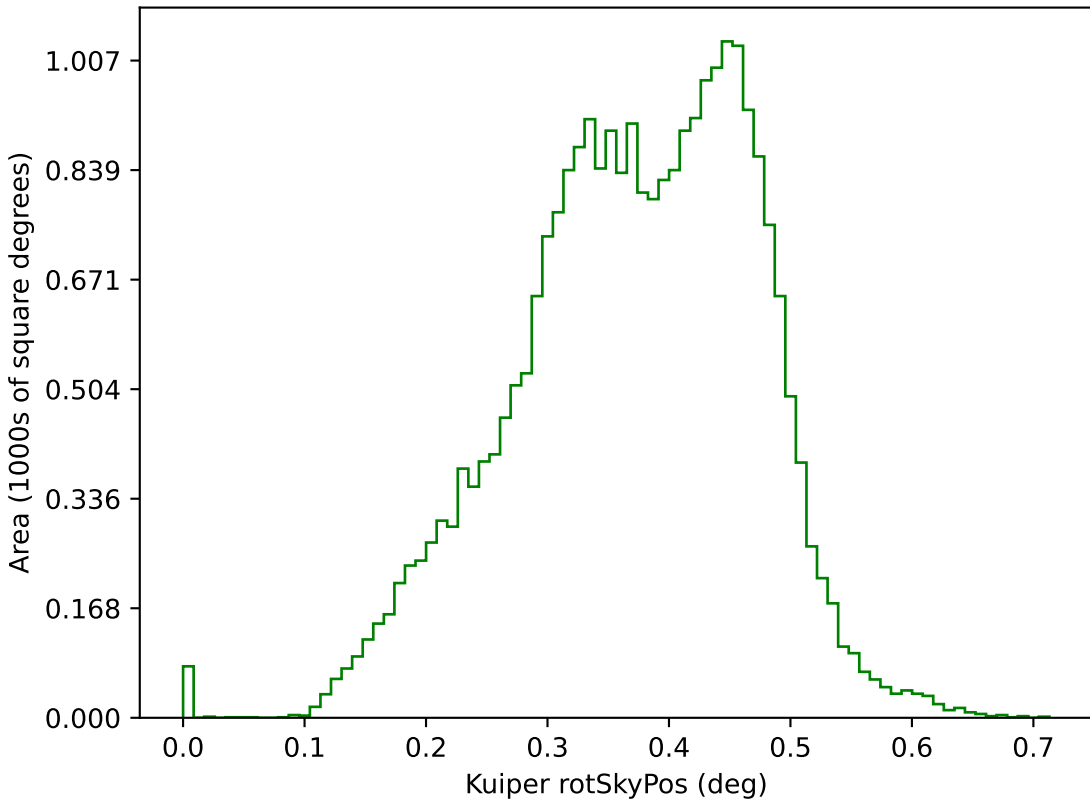
too_elab_r8_d2_giz_v3.4_10yrs g: Kuiper rotSkyPos
