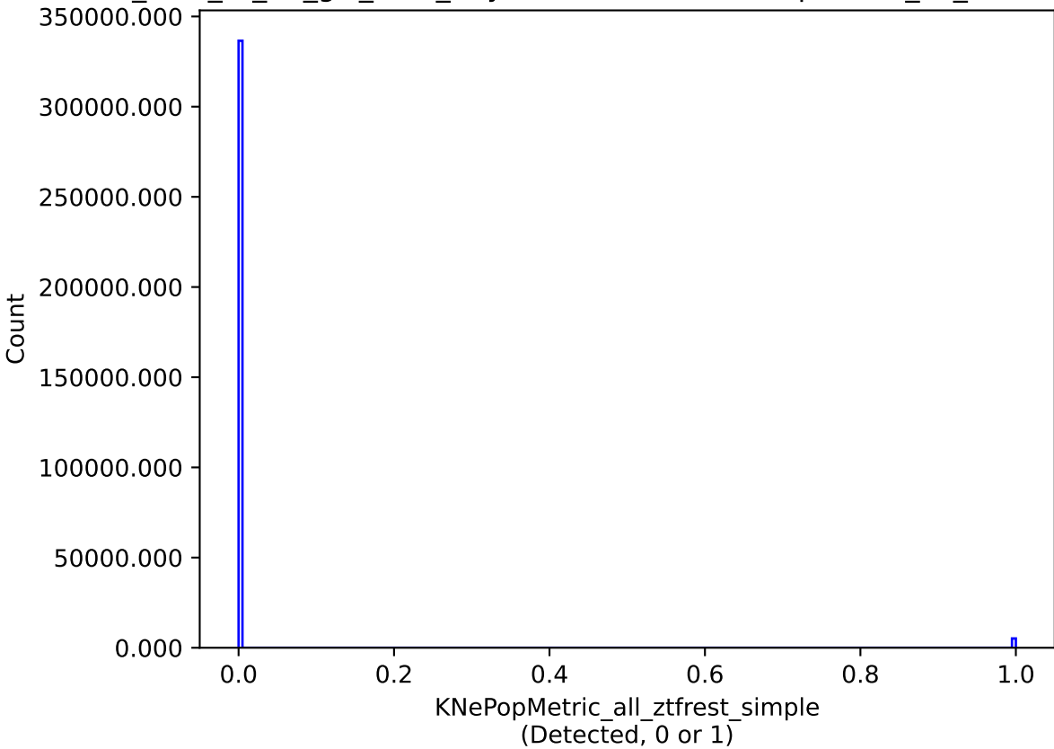
too_elab_r8_d2_giz_v3.4_10yrs all models: KNePopMetric_all_ztfrest_simple
