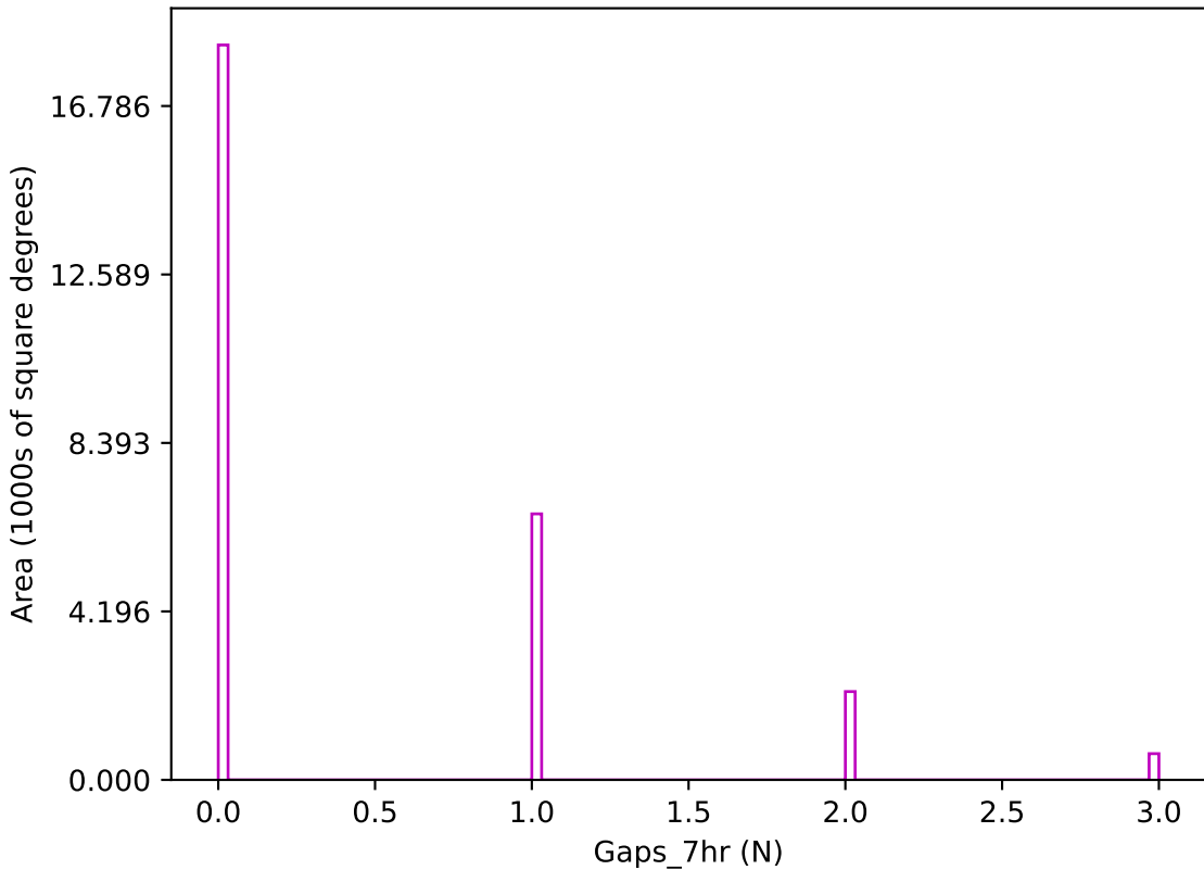
too_elab_r8_d2_giz_v3.4_10yrs z band: Gaps_7hr
