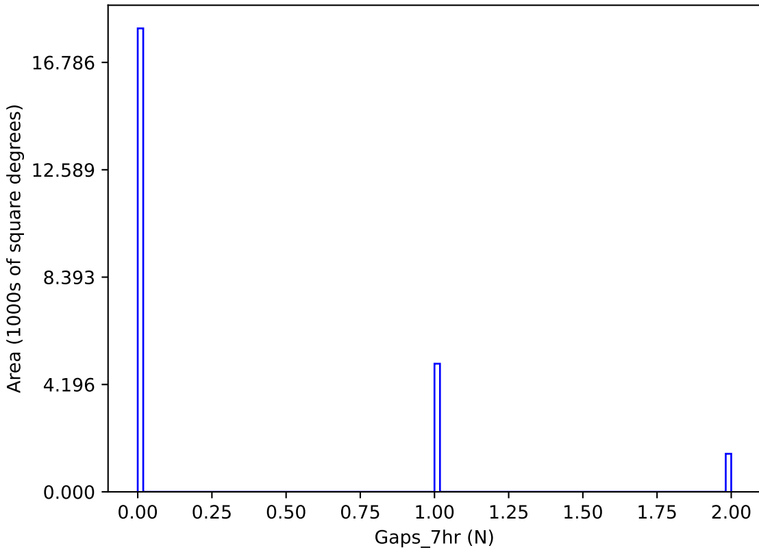
too_elab_r8_d2_giz_v3.4_10yrs y band: Gaps_7hr
