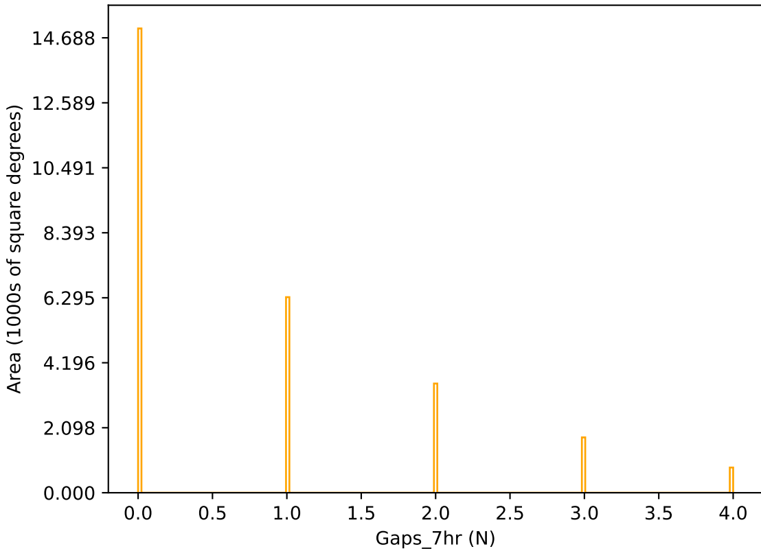
too_elab_r8_d2_giz_v3.4_10yrs r band: Gaps_7hr
