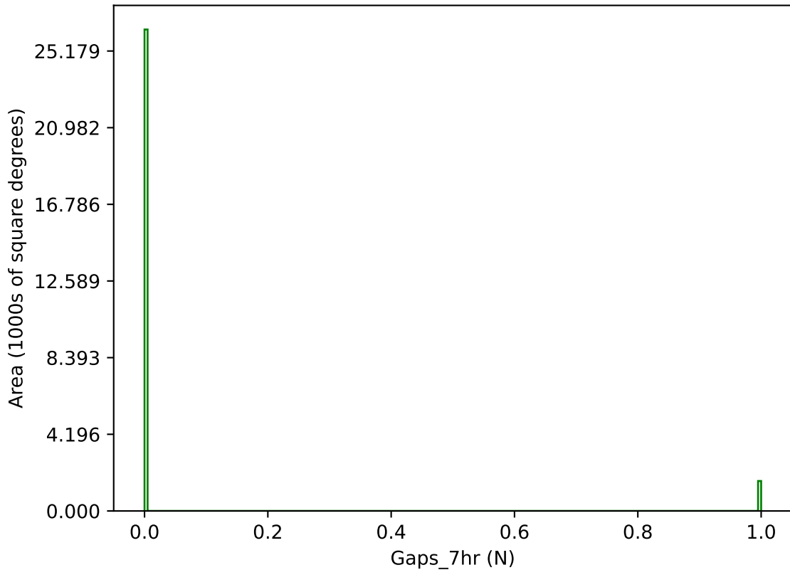
too_elab_r8_d2_giz_v3.4_10yrs g band: Gaps_7hr
