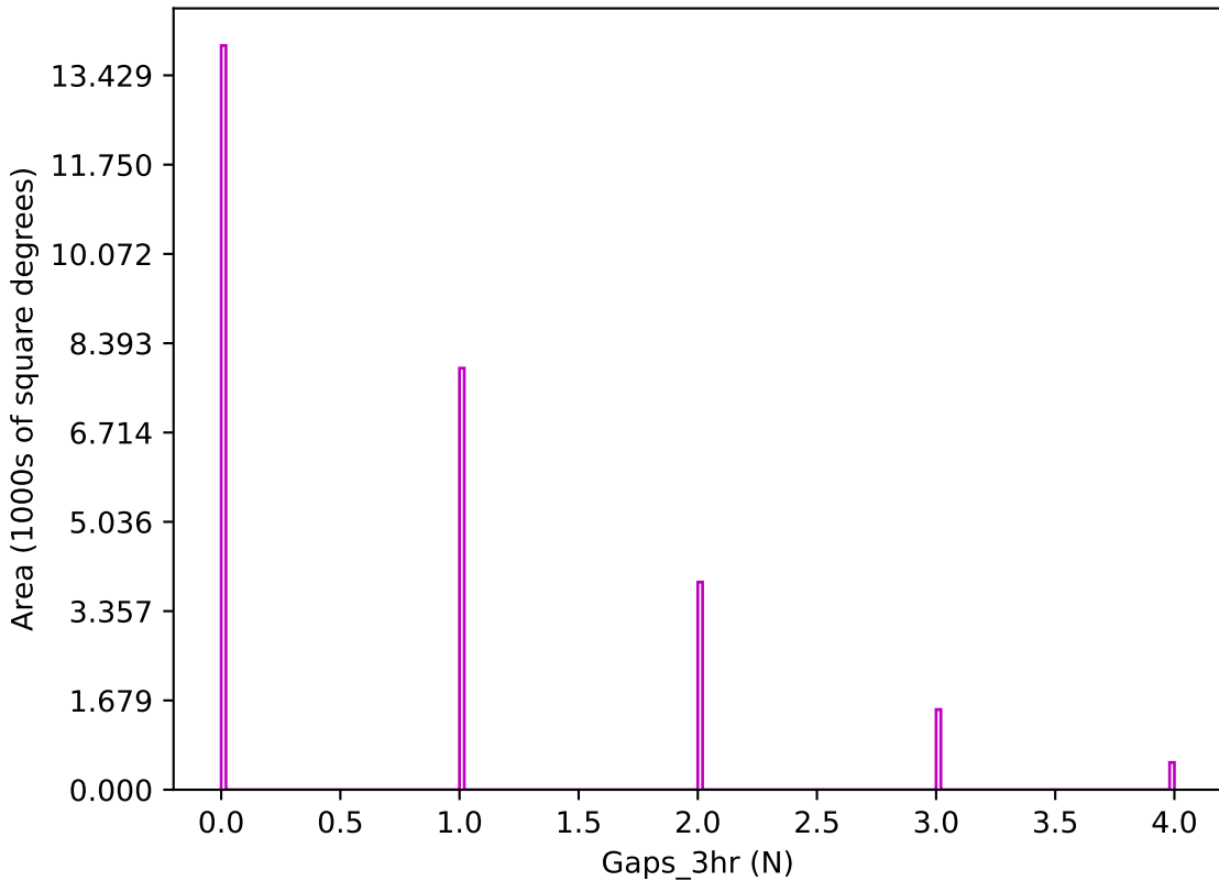
too_elab_r8_d2_giz_v3.4_10yrs z band: Gaps_3hr
