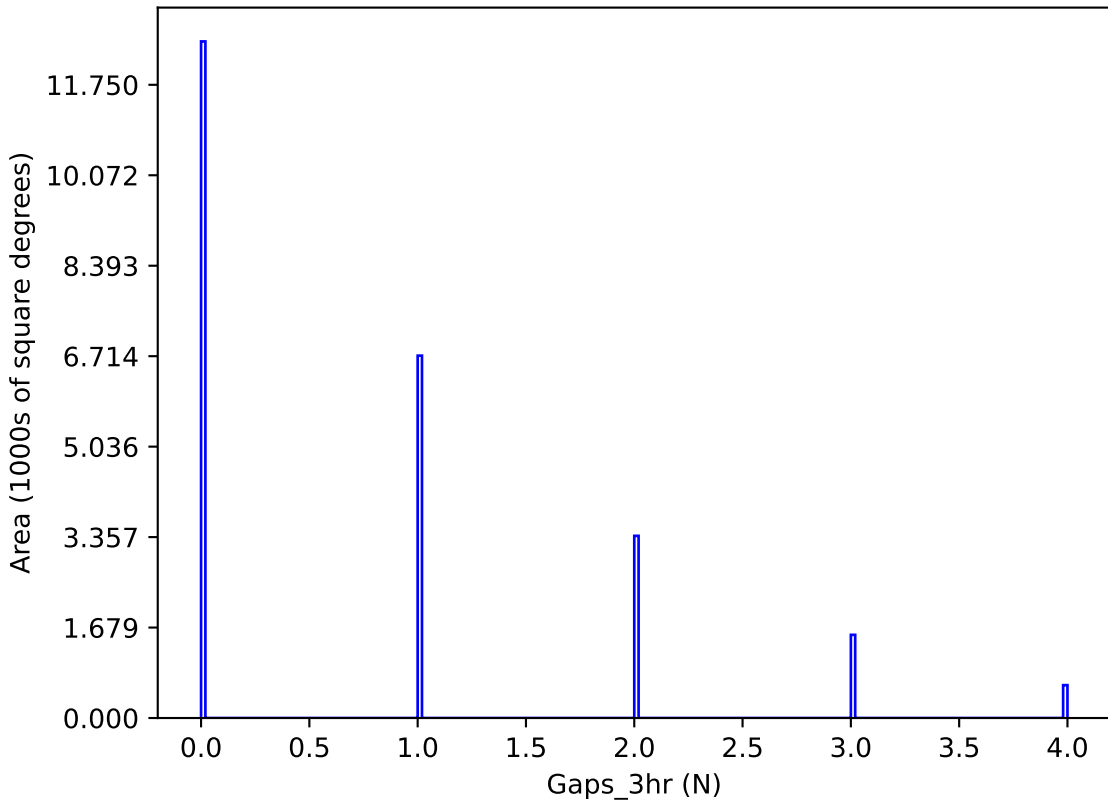
too_elab_r8_d2_giz_v3.4_10yrs y band: Gaps_3hr
