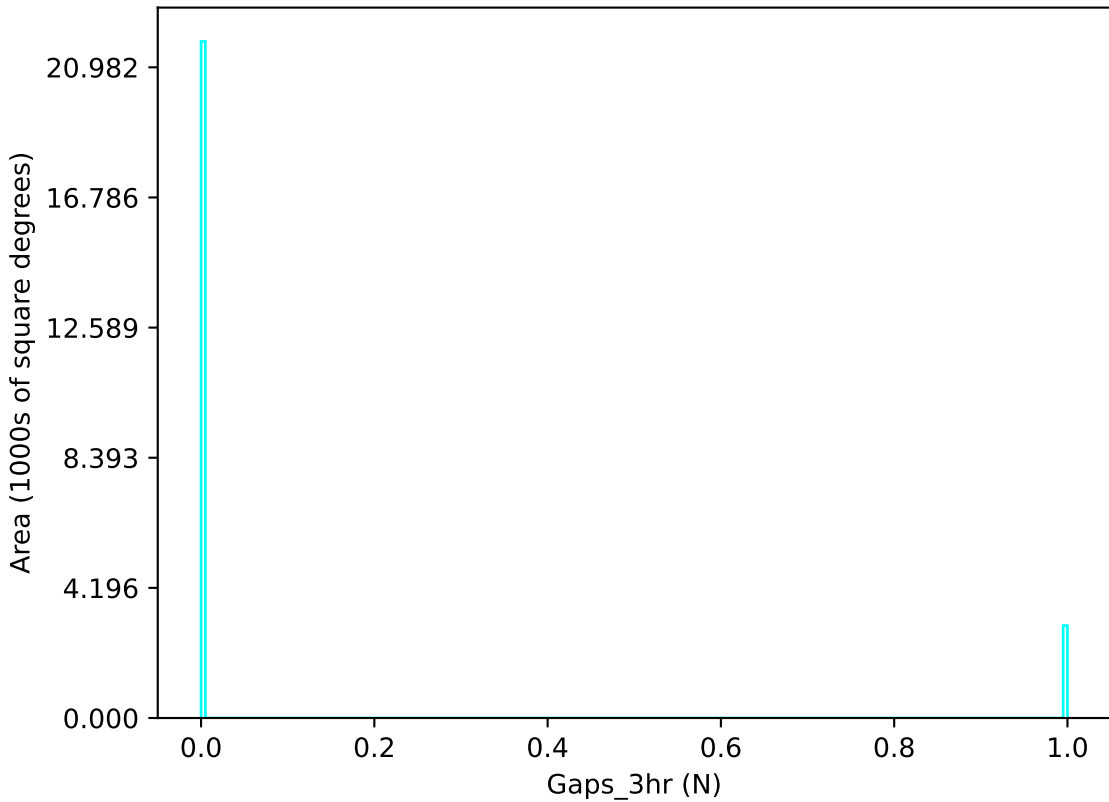
too_elab_r8_d2_giz_v3.4_10yrs u band: Gaps_3hr
