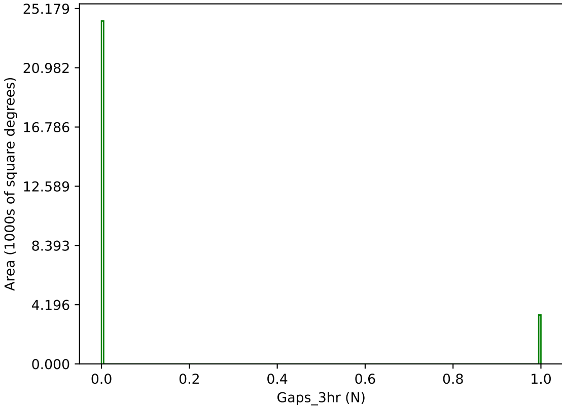
too_elab_r8_d2_giz_v3.4_10yrs g band: Gaps_3hr
