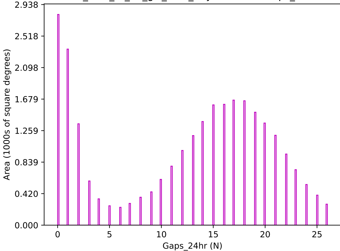
too_elab_r8_d2_giz_v3.4_10yrs z band: Gaps_24hr
